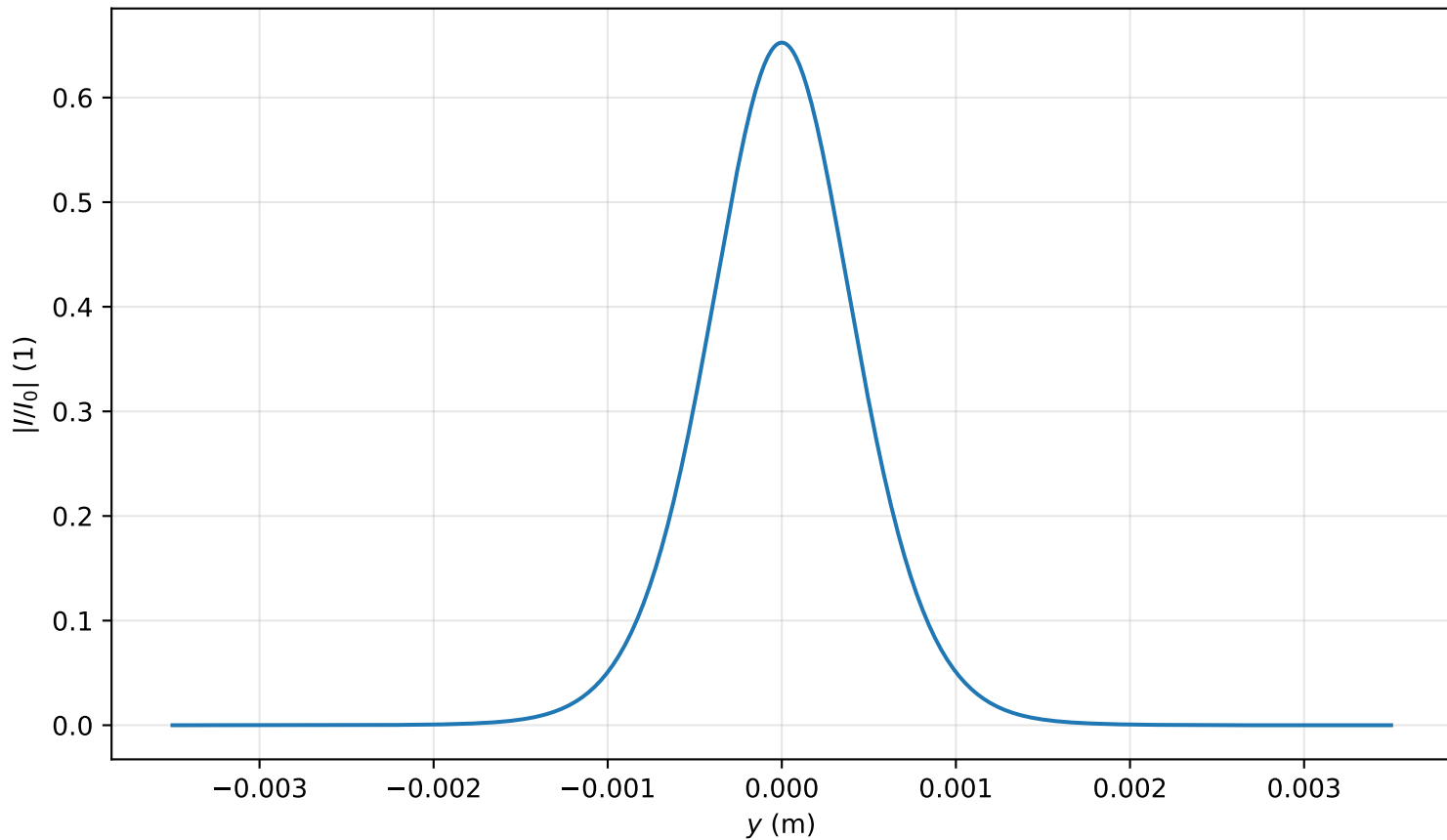
Intensity profile I(x=0, y, z=2.627)/I_0 , \text{Pin}=0.5\text{Pcr} , artificial time
